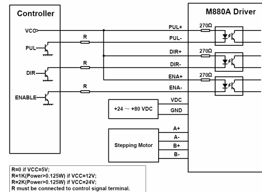
Figure 10: Typical connection
