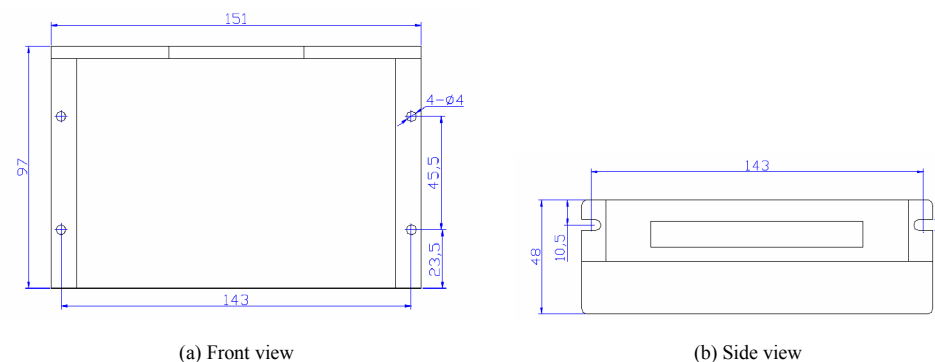
Figure 1: Mechanical specifications
